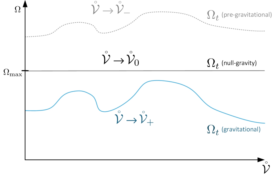
Figure 8: Vacuum States
