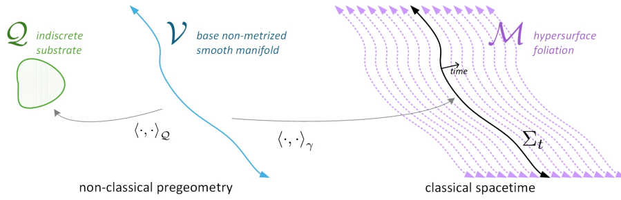
Figure 1: Bitopological Framework
