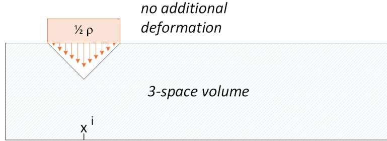
Figure 4: Dark Matter
