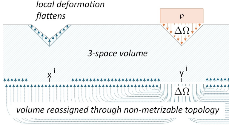
Figure 5: Dark Energy
