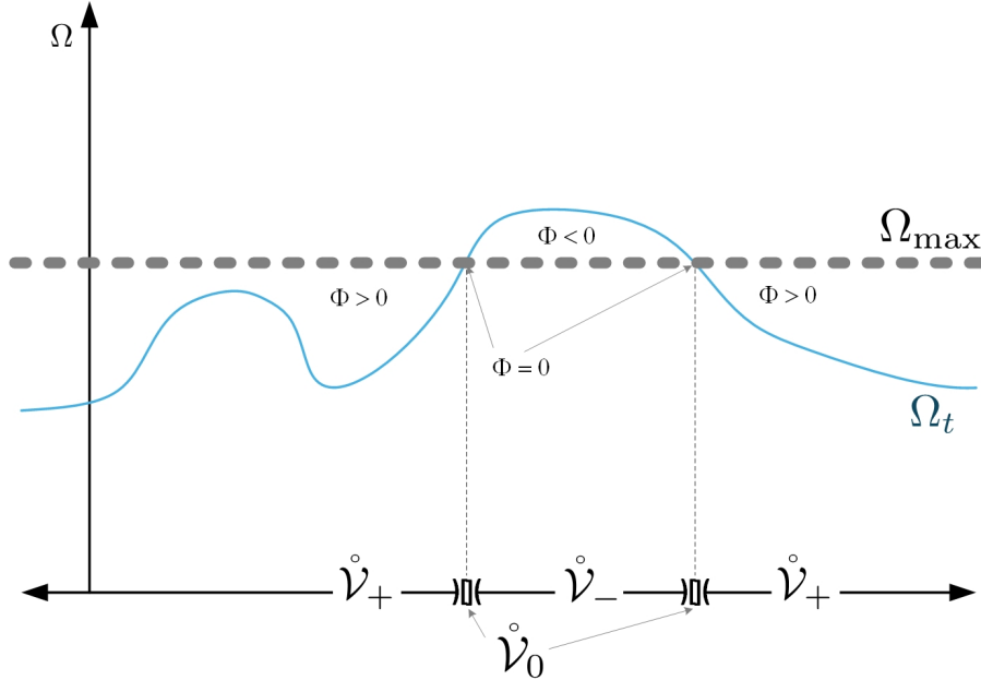
Figure 7: Vacuum Spacetime
